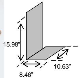
Evaporator Dimensions (Same as SCQT 4407)
