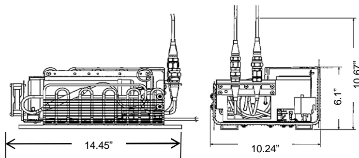
Cooling Unit Dimensions
